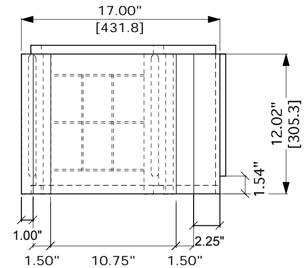
END ELEV,
