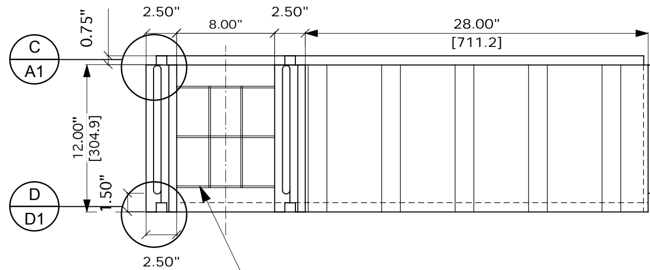
FRONT ELEV,
