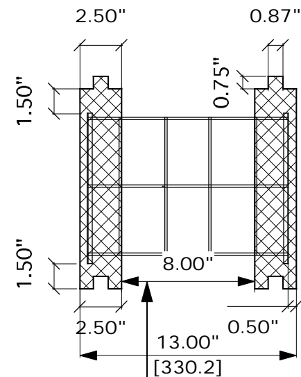
SECTION A
