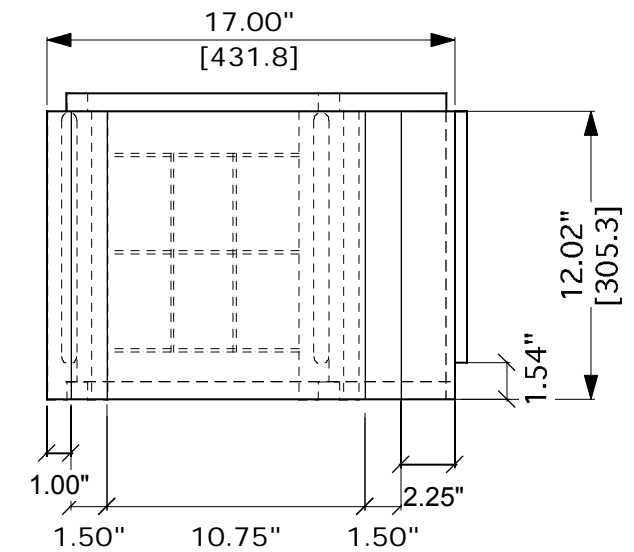
END ELEV,
