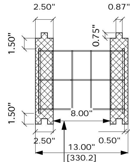
SECTION A
